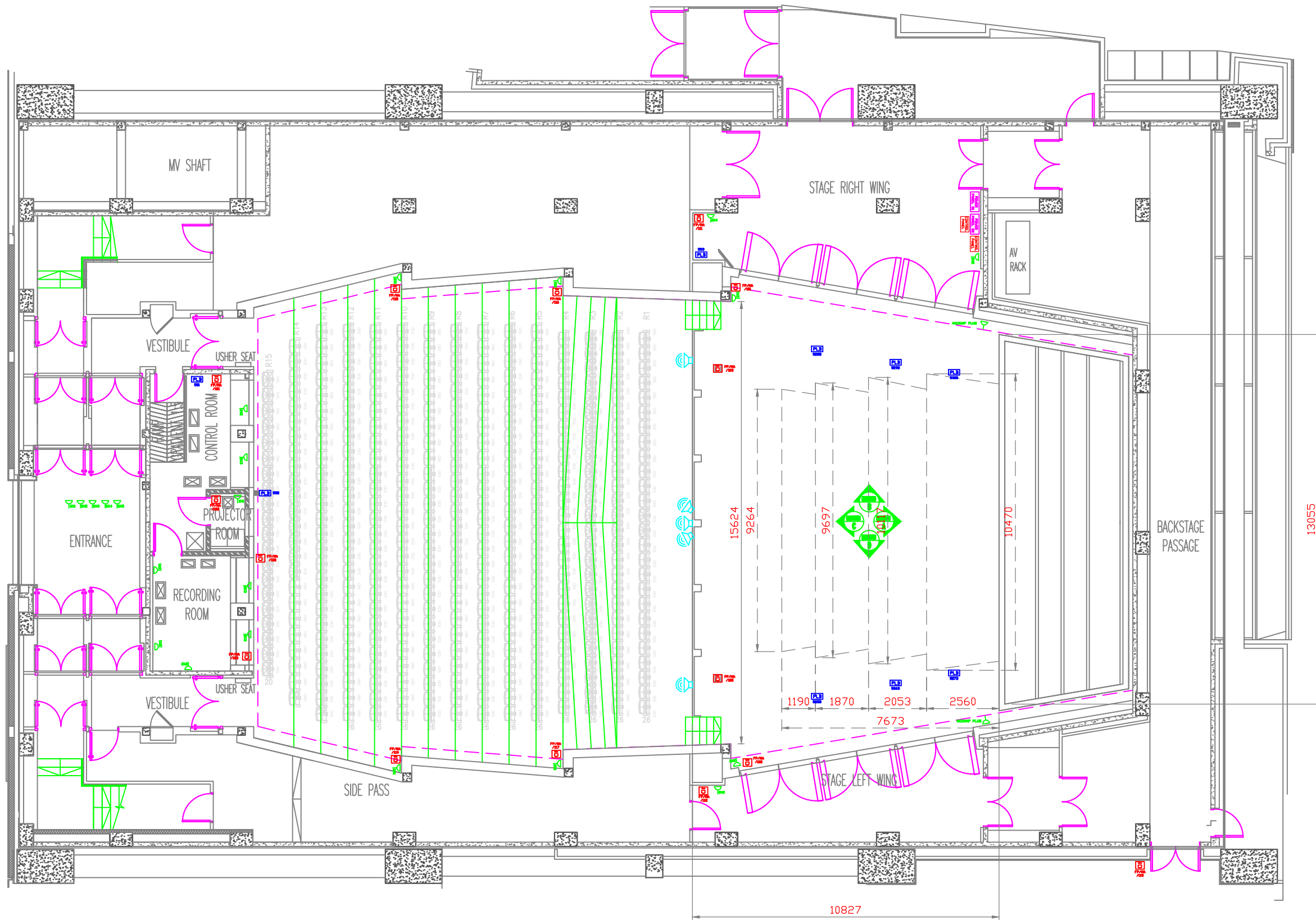
STAGE LEVEL LAYOUT SCALE 1:150
